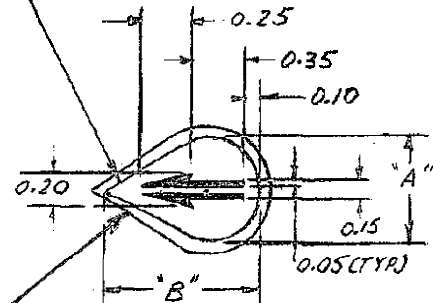
DETAIL OF -2 (SCALE 1:1)
