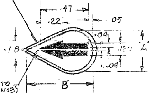
DETAIL OF -4 (SCALE 2:1)
