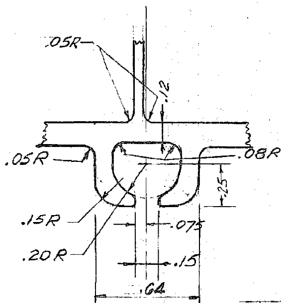
DETAIL "A" TWICE FULL SIZE
