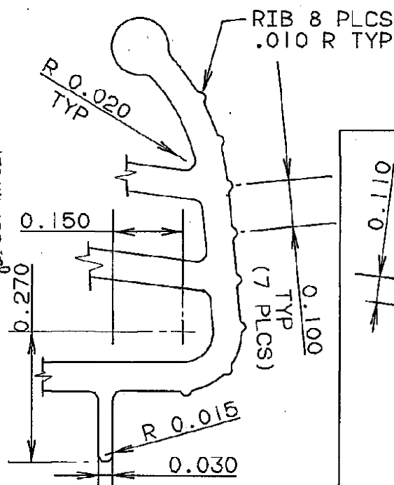
RIB DETAIL SCALE 4:1
