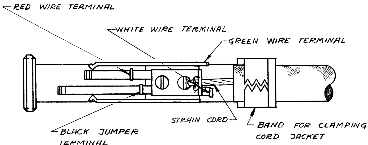
PLUG CONNECTOR U-94/U DETAILS &amp; WIRE CONNECTIONS
