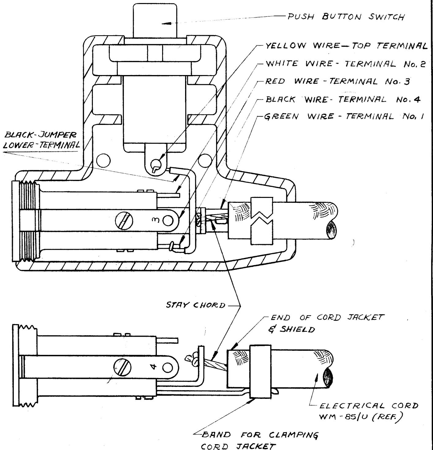
PLUG CONNECTOR U-94 A/U DETAILS &amp; WIRE CONNECTIONS
