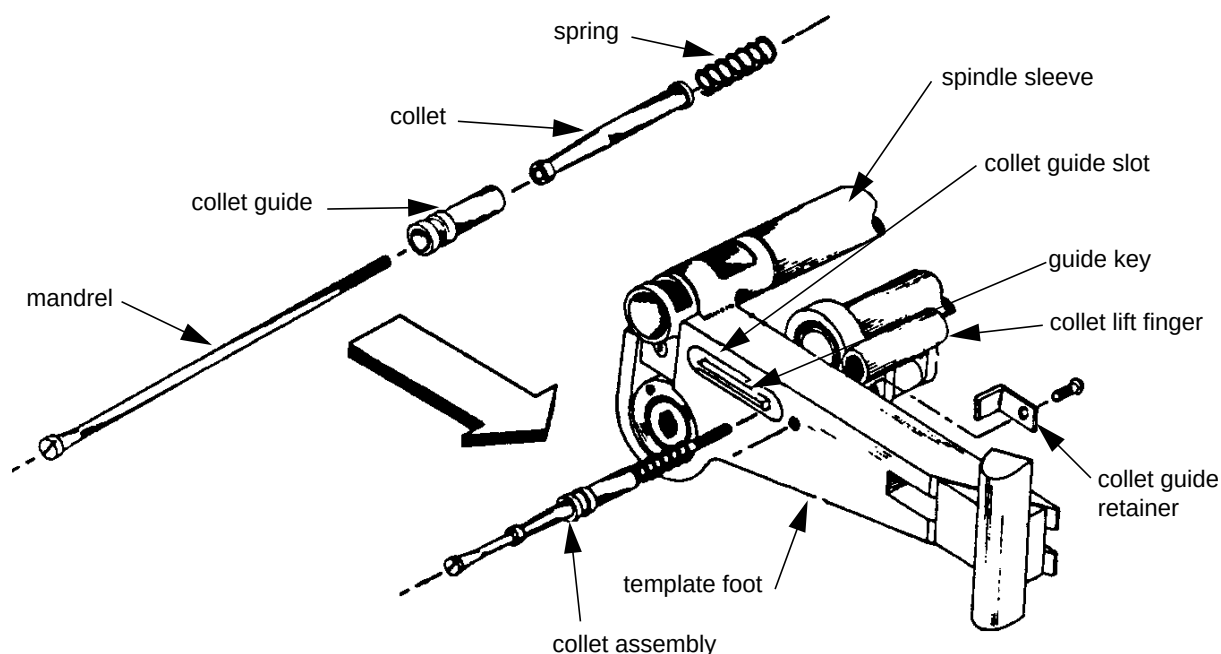
Figure 2 - Installation of Collet Assembly
