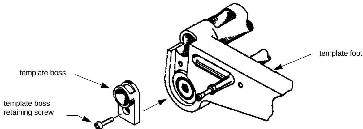
Figure 4 - Installation of Template Boss
