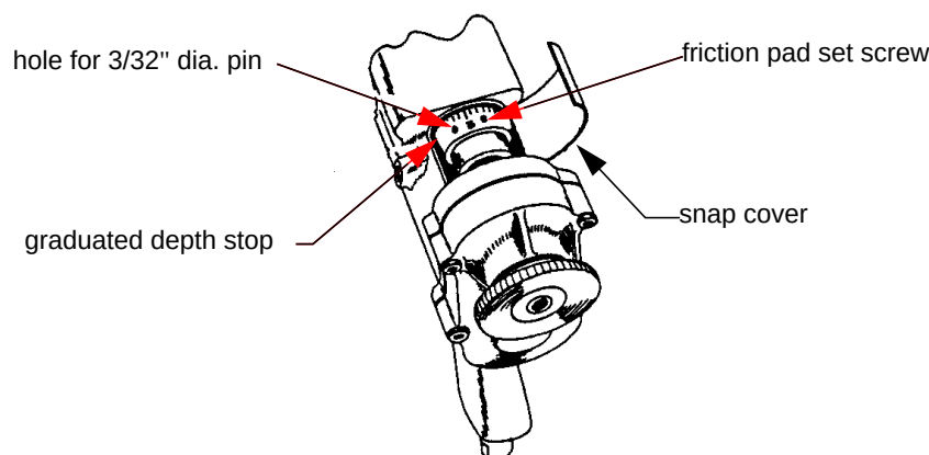
Figure 7 - Drill/Countersink Depth Adjustment
