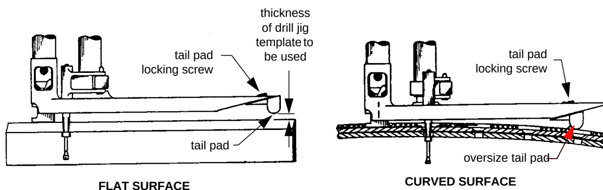
Figure 8 - Tail Pad Adjustment
