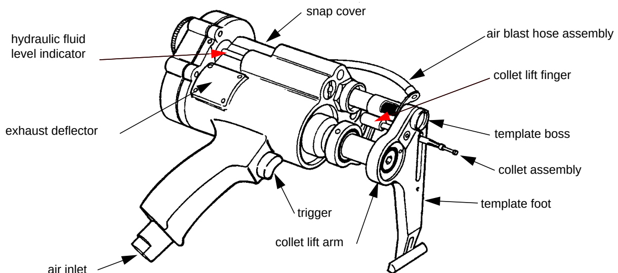
Figure 1 - General Description of Spacematic Drillmotor
