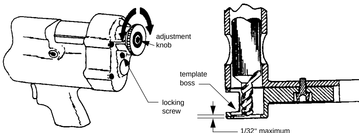
Figure 6 - Drill Point to Work Surface Adjustment
