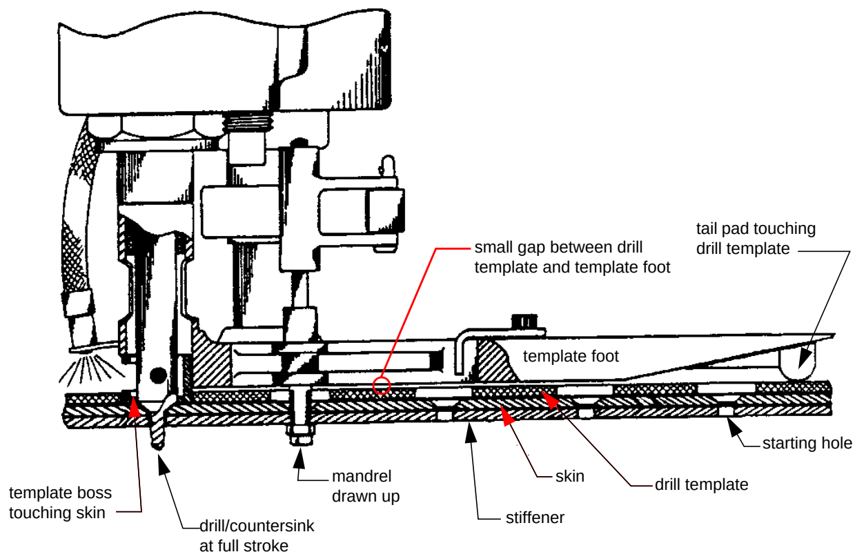
Figure 11 - Typical Drill Countersinking Operation
