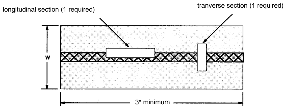
Figure 1 - Nugget Diameter and Macroscopic Examination Test Specimen (Spot and Intermittent Spot welds)
